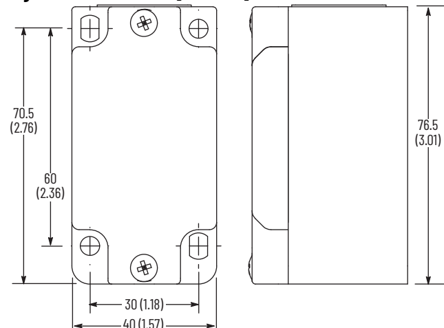
Figure 59 - Dimensions [mm (in.)]
