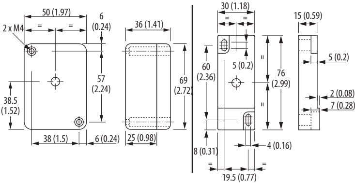
Figure 35 - Interlock Switch Dimensions [mm (in.)]
